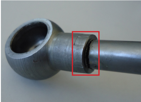
Example of fatigue rupture in the banjo-pipe junction area
