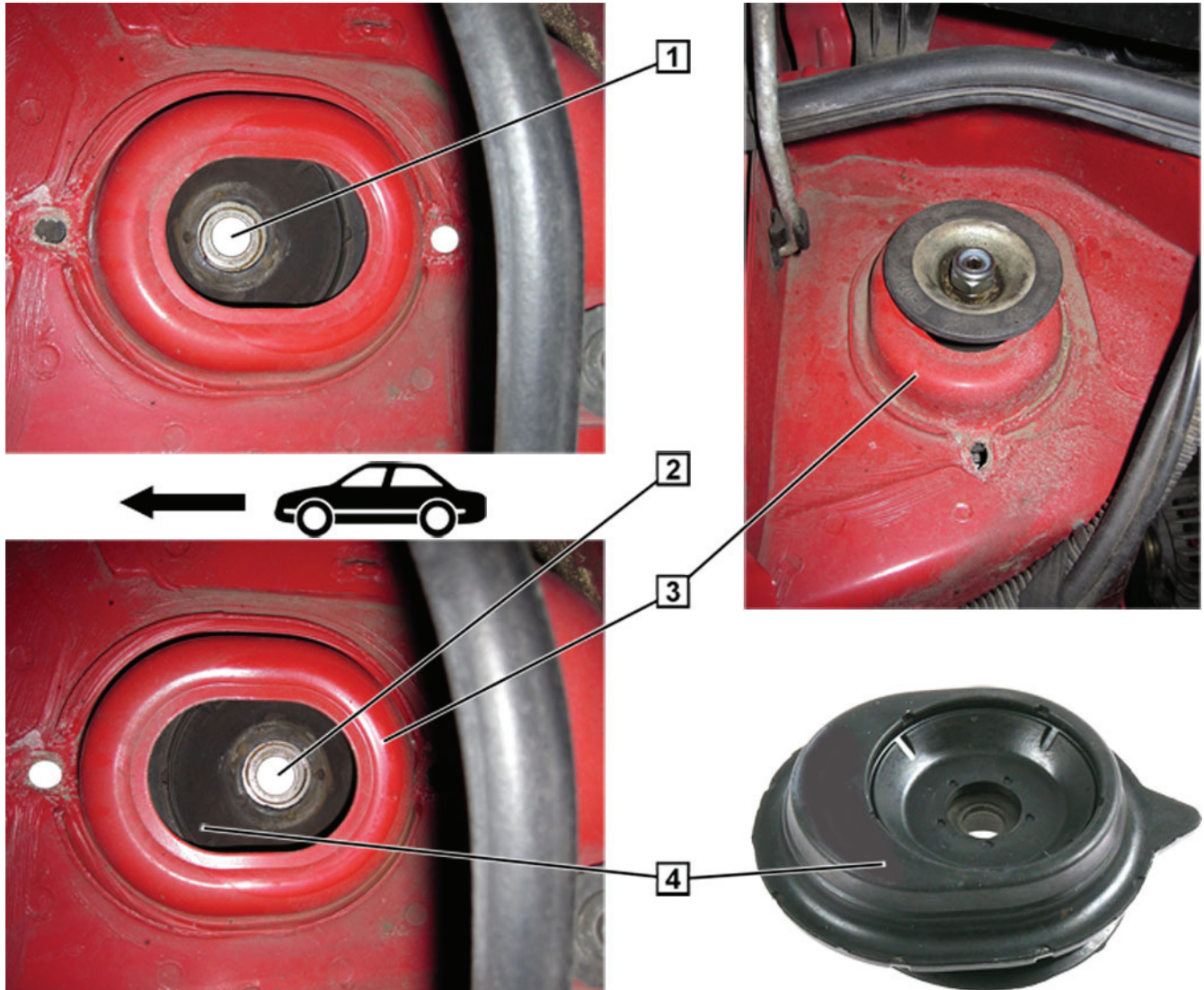
Fig. 1: Suspension strut mount in different installation positions
