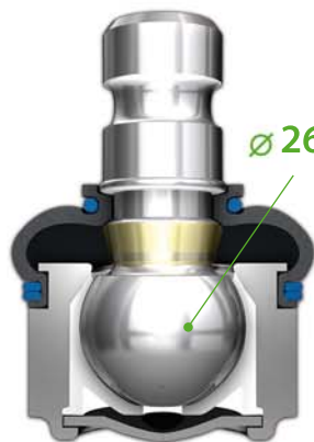
Enlarged ball diameter in ball joint
